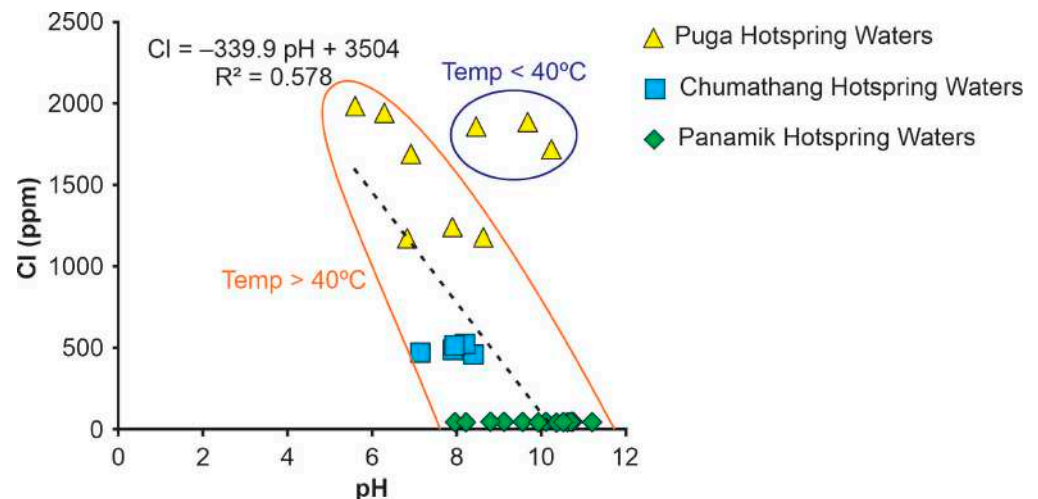
Figure 7. The Cl vs. pH plot shows a significant negative correlation between the two parameters for the hotspring waters having temperature > 40 °C. The Pearson coefficient for the regression equation is found to be < 0.05 .
