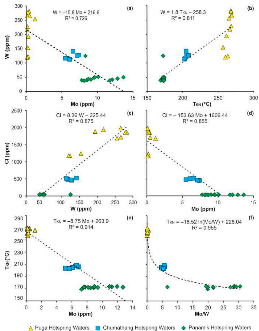
Figure 2. The cross plots of (a) W vs. Mo, (b) W vs. TKN, (c) Cl vs. W, (d) Cl vs. Mo, (e) TKN vs. Mo, and (f) TKN vs. Mo/W with their respective R 2 values and regression equations. The Pearson coefficient for each regression equation is found to be <0.05.
